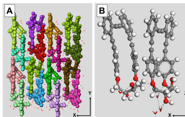
Fig. 3 (A) Top view of a monolayer of ( R,R,M )- 1 molecules onto a water surface. XYZ dimension values of the computational box were 24 \times 30 \times 150 \text{ \AA}^3 . Water molecules are depicted as sticks for clarity. (B) Close detail of ( R,R,M )- 1 molecules in the monolayer. Additional ( R,R,M )- 1 and water molecules are omitted for clarity. The formation of intermolecular H-bonds between neighbour ( R,R,M )- 1 molecules and H-bonds with water is displayed as a dashed black line, left and right, respectively.
