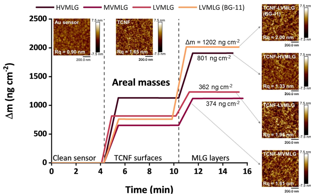
Fig. 5 Adsorbed MLG layers at the solid–air interface. Areal masses of clean sensors, added TCNF layers, as well as different MLG layers on TCNF surfaces. 15 MHz, f_0 = 5 MHz, n = 3 . Layer density assumed as 1.05 \text{ g cm}^{-3} . Final \Delta m between TCNF and TCNF–MLG surfaces are given. 1 \times 1 \mu\text{m} AFM height images of the corresponding surfaces are included for visual representation and the clean Au sensor is shown as a reference. The images were flattened and analysed with NanoScope Analysis software (Bruker), and the root-mean-square roughness ( R_q ) values of each surface are embedded in the images.
