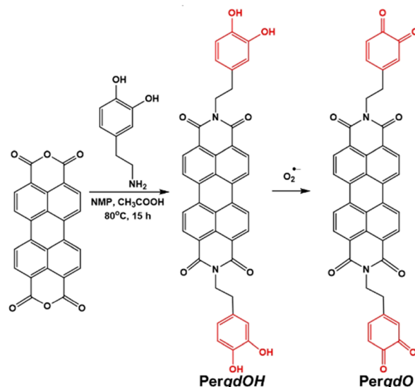
Scheme 1 The synthesis route of P-OH and its interaction with O_2^{\bullet-} .
