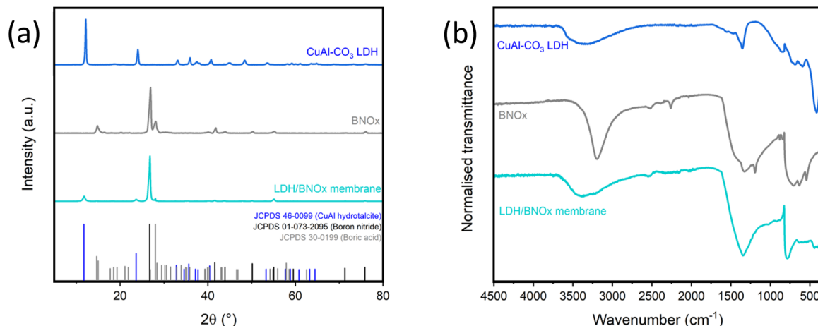
Fig. 1 (a) pXRD patterns and (b) FT-IR spectra of CuAl-CO 3 LDHs (blue), BNOx (grey) and LDH/BNOx nanocomposite (turquoise). pXRD reference patterns are provided for CuAl hydrotalcite, boron nitride and boric acid.
