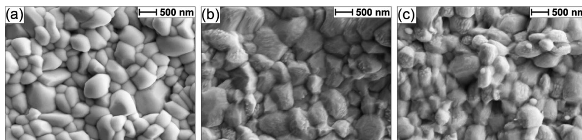
Fig. 2 SEM images for an FTO/Ti/Au/ \text{Sb}_2\text{Se}_3 sample (a) untreated, (b) etched via (NH 4 ) 2 S, and (c) etched via (NH 4 ) 2 S + CuCl 2 treatment.
