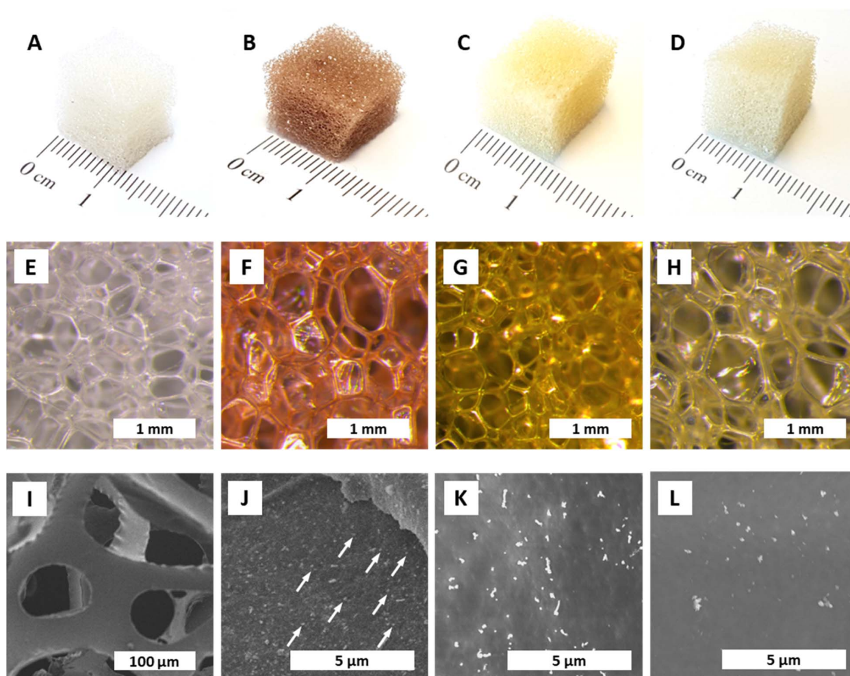
Fig. 1 Aspect and morphology of NPs@PUF. All specimens were synthesized at T_R = 120\text{ }^{\circ}\text{C} , t_R = 3\text{ h} , and [M^{X+}] = 0.25\text{ mM} . Macroscopic aspect (A–D) and optical micrographs (E–H) of pristine PUF and NPs@PUFs: pristine PUF (A and E), AuNP@PUF (B and F); AgNP@PUF (C and G), PdNP@PUF (D,H). SEM micrographs of pristine PUF(I), and NPs@PUFs: AuNP@PUF (J) with some AuNPs indicated with white arrows; AgNP@PUF (K); and PdNP@PUF (L).
