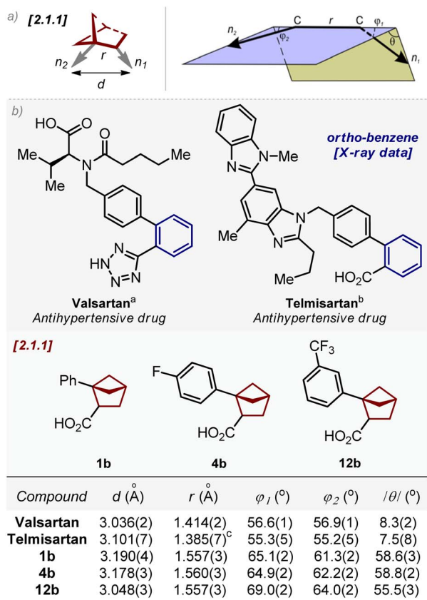
Fig. 3 (a) Definition of vectors n_1 and n_2 , and geometric parameters d , r , \phi_1 , \phi_2 and \theta . 1,2-Disubstituted bicyclo[2.1.1]hexane is shown as an example. (b) Geometric parameters d , r , \phi_1 , \phi_2 , and |\theta| for ortho -substituted benzenes (valsartan and telmisartan); and bicyclo[2.1.1]hexanes 1b, 4b, and 12b. a Data are taken from ref. 25a. b Data are taken from ref. 25b. c Two molecules of telmisartan are present in the crystalline lattice with r = 1.385(7) Å and 1.395(7) Å (ref. 25b).
