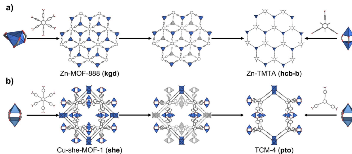
Fig. 3 Schematic of the net-clipping approach applied to formation of reticular materials from (a) hexagonal CPB linker to a trigonal TMTA linker combined with 3- c Zn(II) MBBs; and (b) from a hexagonal BHEB linker to a trigonal BTEB combined with 4- c paddlewheel Cu(II) MBBs.
