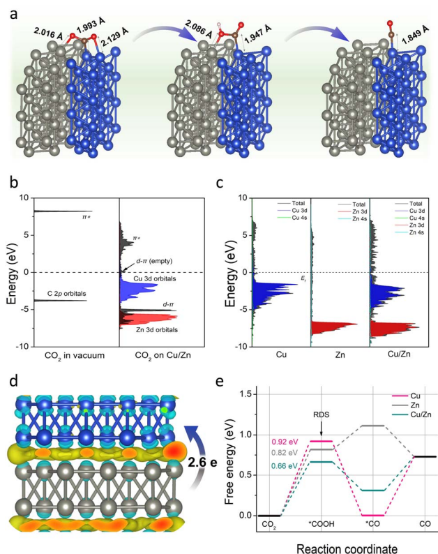
Fig. 4 (a) The adsorption state of CO 2 , *COOH, and *CO on the Cu/Zn-CP-1-30 electrode. The blue, gray, brown, red, and white balls represent Cu, Zn, C, O, and H atoms, respectively. (b) Projected electronic densities of states of the C 2p orbitals of CO 2 in a vacuum, and the Cu 3d/Zn 3d orbitals and the C 2p orbitals of CO 2 adsorbed on Cu/Zn heterostructures. (c) Densities of states of Cu-CP, Zn-CP, and Cu/Zn-CP heterostructures. (d) Top view of the charge density difference of Cu/Zn hetero-interfaces with an isosurface of 3.6 \times 10^{-3} \text{ e } \text{\AA}^{-3} . (The charge accumulation is shown as the yellow region, and the charge depletion is shown as the cyan region.) (e) Gibbs free-energy diagrams for ECR to CO over the simulated Cu/Zn-CP-1-30 electrode.
