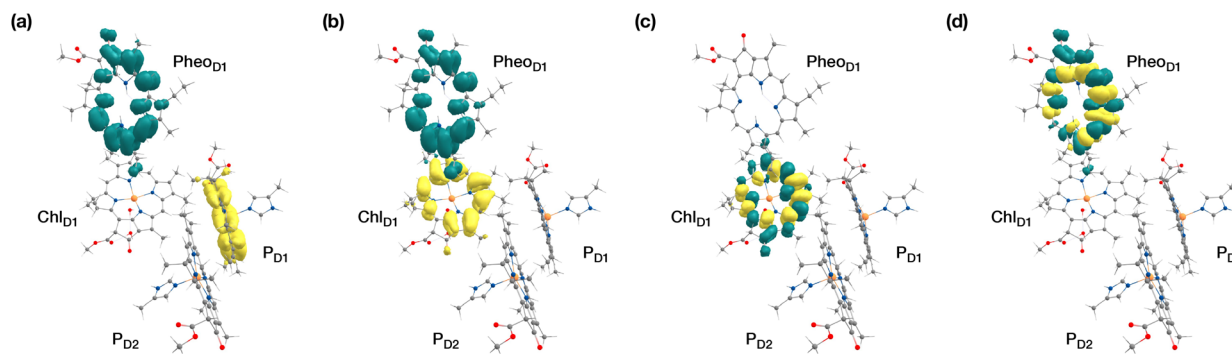
Fig. 5 Difference density isosurfaces describing the lowest singlet-triplet excitations of the D1 branch in PSII: (a) the lowest triplet excitation with ^3[\text{P}_{\text{D1}}^{\delta+}\text{Pheo}_{\text{D1}}^{\delta-}] charge transfer character; (b) the lowest triplet excitation with ^3[\text{Chl}_{\text{D1}}^{\delta+}\text{Pheo}_{\text{D1}}^{\delta-}] charge transfer character; (c) local ^3\text{Chl}_{\text{D1}} excitation; (d) local ^3\text{Pheo}_{\text{D1}} excitation.
