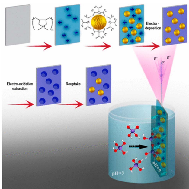
Fig. 14 Schematics of the NAIM electrochemical sol–gel deposition system. First, ITO substrate is treated with PDPA followed by adsorption of AuNPs-cit. Then, the desired silane is electrodeposited on the electrode to form the NAIM. Reprinting (adapted) with permission from ref. 152. Copyright 2018, the American Chemical Society.
