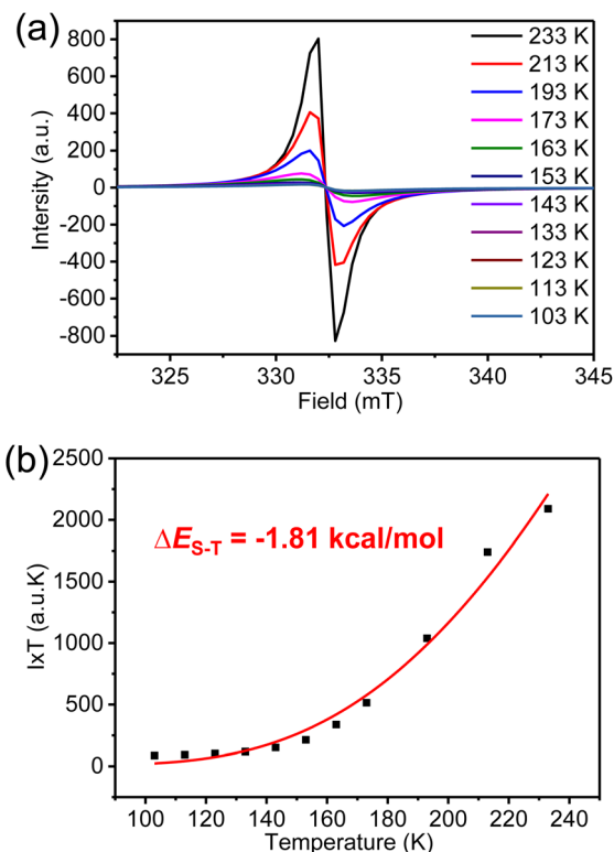
Fig. 6 (a) VT ESR spectra and (b) fitted \ln T vs T-T curves by using the Bleaney–Bowers equation of carbonylated cycloarene diradical K3-R in a solid.
