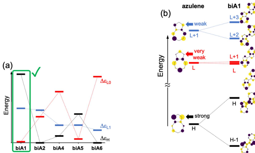
Fig. 3 (a) Orbital energy differences ( \Delta\epsilon_H , \Delta\epsilon_{L1} , and \Delta\epsilon_{L0} ) for symmetrical biazulenes (biA1–biA6). (b) Molecular orbital diagrams of azulene and biA1. Participation of p z -orbital in position 1 of azulene highlighted. Energy gaps and orbitals obtained with the Hückel model. H = HOMO; L = LUMO.
