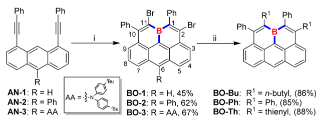
Scheme 1 Synthetic routes toward 11a-boraolympicenes. Conditions: (i) \text{BBr}_3 , toluene, reflux; (ii) tetrabutyltin or tributylphenylstannane or 2-(tributylstannyl)thiophene, \text{Pd(PPh}_3)_4 , CuI, toluene, reflux.
