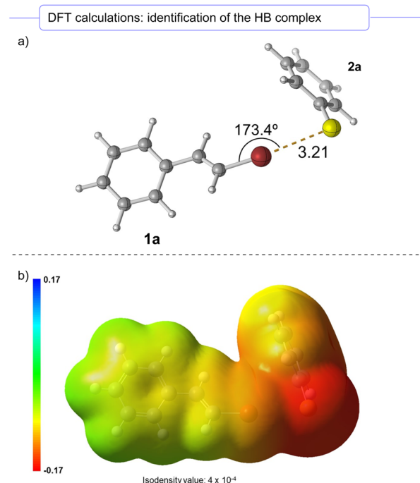
Scheme 5 (a) HB complex between 1a and the anionic form of 2a calculated at the \omega B97x-D3/Def2TZVPP. (b) Calculated electrostatic potential (red = negative electrostatic potential) on the 0.0004 au isodensity surface.
