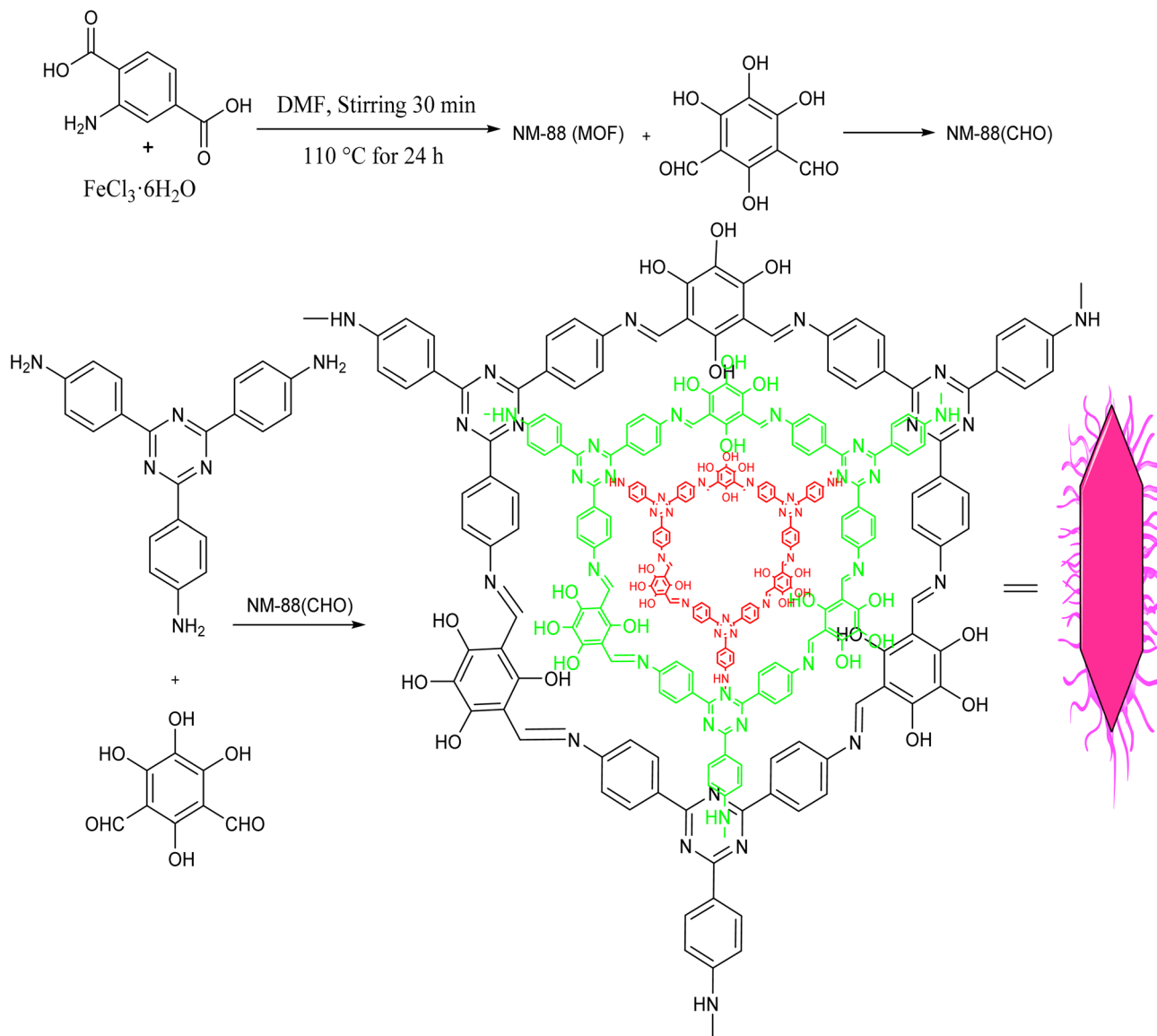
Fig. 9 The preparation of NMC Tp-TPA hybrid nanozyme. Reproduced with permission from ref. 22.
