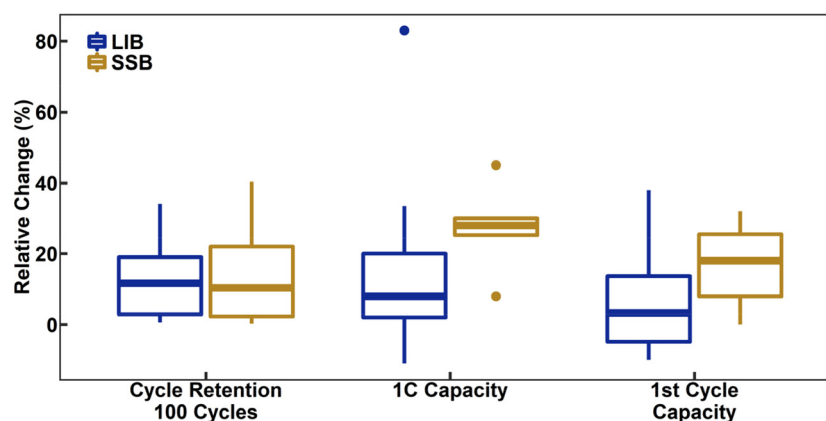
Fig. 5 Box-and-whisker plot of the relative change of capacity retention after 100 cycles, 1C capacity, and first-cycle capacity of LiNbO 3 coatings with respect to “bare” NCM CAMs for both LIB and SSB systems. For cycle retention, n = 19 and 9 for LIB and SSB, respectively. For 1C capacity, n = 17 and 6 for LIB and SSB, respectively. For first-cycle capacity, n = 18 and 11 for LIB and SSB, respectively.
