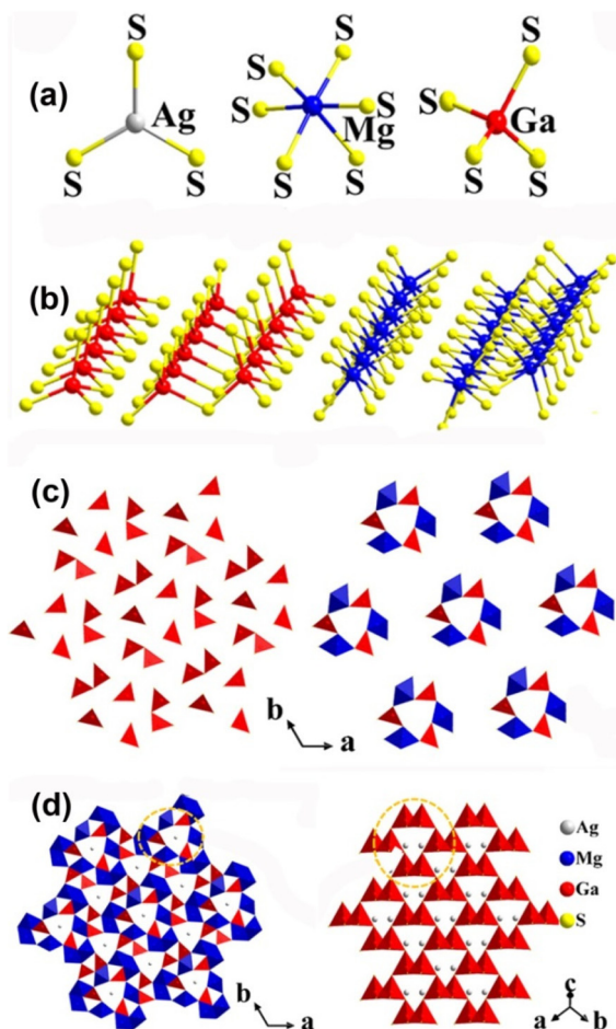
Fig. 11 (a) Coordinated environment of [\text{AgS}_3] , [\text{MgS}_6] , and [\text{GaS}_4] atoms; (b) 1D [\text{GaS}_4] , [\text{Ga}_2\text{S}_7] , [\text{MgS}_6] , and [\text{Mg}_2\text{S}_5] chains; (c) 1D Ga–S chains and [\text{Mg}_3\text{Ga}_3\text{S}_{24}] groups viewed along the ab plane; (d) 3D structure of \text{AgMg}_3\text{Ga}_2\text{S}_8 (left) and \text{AgGaS}_2 (right) with the [\text{Ga}_6\text{S}_{18}] units marked (yellow dashed circle). Copyright 2022 American Chemistry Society.
