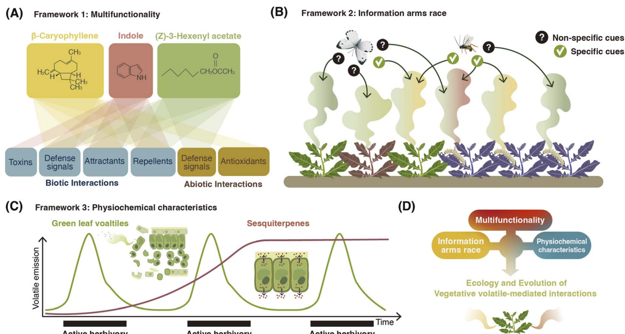
Fig. 5 Biological frameworks that help to explain release patterns of vegetative plant volatiles. (A) Multifunctionality: plant volatiles can serve multiple purposes for plants, and this multifunctionality is mirrored in the regulation of their production and release. (B) Vegetative volatiles provide information to both allies and antagonists, which may result in an information arms race that shapes the composition of plant volatile bouquets. Different colors depict different blends of volatiles, some of which contain useful information only for beneficials and others can act as useful signals for both beneficials and enemies. (C) Physiochemical characteristics such as the biochemical origin, the volatility, the stability and the toxicity of vegetative volatiles influence their production and release kinetics, which again determines potential functions and environmental effects. (D) Interactions between A, B, and C will influence the evolution of vegetative plant volatiles, and thus help to explain spatiotemporal production and release patterns that are observed in nature.
