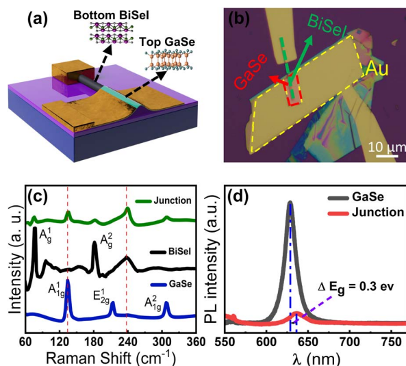
Fig. 1 (a) The 3D diagram of the BiSel/GaSe heterostructure photo-detector. (b) Optical microscopy image and (c) Raman spectra of individual BiSel, GaSe and the BiSel/GaSe heterojunction under 532 nm laser excitation. (d) Photoluminescence spectra of individual GaSe and the BiSel/GaSe heterojunction.
