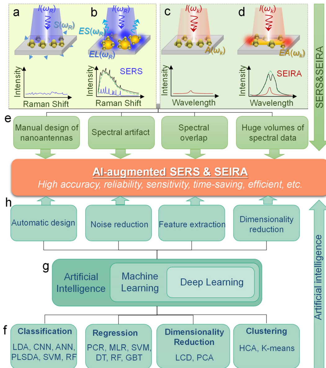
Fig. 2 Concept of machine learning-enhanced SERS and SEIRA. (a) Conventional Raman scattering S_{\omega} , and Raman spectrum with incident radiation R_{\omega_0} . (b) Surface-enhanced Raman scattering using nanoparticle substrates. Enhanced local field ( EL_{\omega_0} ) is achieved by utilizing the localized surface plasmon polariton (LSP) of nanoparticles, and then the excitation and radiation efficiency of Raman scattering is improved by the interaction with LSP, which is expressed as ES_{\omega} . (c) Conventional IR absorption and spectrum A_{\omega_0} of molecules with incident IR radiation I_{\omega_0} . (d) Surface-enhanced infrared absorption. Enhanced absorption of molecules ( EA_{\omega_0} ) is realized by the near-field coupling of LSP and molecules. (e) Challenges and issues of SEIRA and SERS. (f) Model categories of machine learning for SERS and SEIRA. (g) Relationship between AI, ML, and DL. (h) Benefits of ML brought to SERS and SEIRA.
