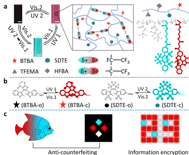
Fig. 1 Concept and preparation of PSFPs . (a) Schematic illustrations of the design strategy from two photochromic fluorescent monomers to a photoswitchable multistate fluorescent polymer, and dipole-dipole interactions based on a strong molecular dipole. Scale bar: 1.0 cm. (b) Schematic diagram of light-induced reversible structural transformation of BTBA and SDTE (non-emission, red and green). UV1: 365 nm; Vis1: 525 nm; UV2: 254 nm; Vis2: 460 nm. (c) Schematic illustration of an example underwater application (anti-counterfeiting, information encryption).
