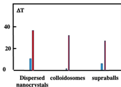
Fig. 14 Temperature in solution induced by subjecting the superstructures and dispersed Fe 3 O 4 nanocrystals (blue) and in a pellet of 1 million cells having internalized Fe 3 O 4 nanocrystals, colloidosomes and supraballs (red). Dispersion in 100 \mu L of phosphate-buffered saline upon irradiation with an 808 nm laser (1 W cm -2 ) for 5 min.
