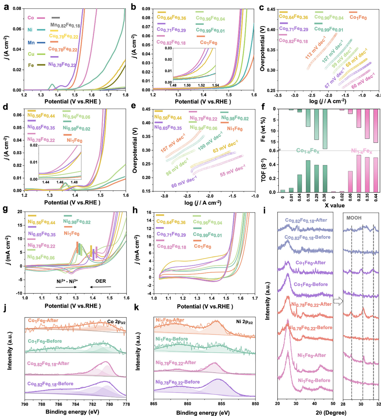
Fig. 3 Electrocatalytic performance of synthesized MFe-LDHs. (a) Polarization curves at 5 \text{mV s}^{-1} for different MFe-LDHs, (b) polarization curves of \text{Co}_{1-x}\text{Fe}_x -LDHs, (d) polarization curves of \text{Ni}_{1-x}\text{Fe}_x -LDHs. (c) Tafel plots of \text{Co}_{1-x}\text{Fe}_x -LDHs, (e) Tafel plots of \text{Ni}_{1-x}\text{Fe}_x -LDHs, (f) verified Fe (wt%) contents from ICP-OES results and the measured TOFs (overpotential = 350 mV) of \text{Co}_{1-x}\text{Fe}_x -LDHs and \text{Ni}_{1-x}\text{Fe}_x -LDHs; (g) 20th scan of cyclic voltammogram of \text{Ni}_{1-x}\text{Fe}_x -LDHs, (h) 20th CV of \text{Co}_{1-x}\text{Fe}_x -LDHs, (i) XRD patterns of Ni, Co, \text{Co}_{0.82}\text{Fe}_{0.18} , and \text{Ni}_{0.78}\text{Fe}_{0.22} before and after the OER process and the enlarged patterns, (j) XPS spectra of Co 2p_{3/2} of Co and \text{Co}_{0.82}\text{Fe}_{0.18} -LDHs, and (k) Ni 2p_{3/2} of Ni and \text{Ni}_{0.78}\text{Fe}_{0.22} -LDHs.
