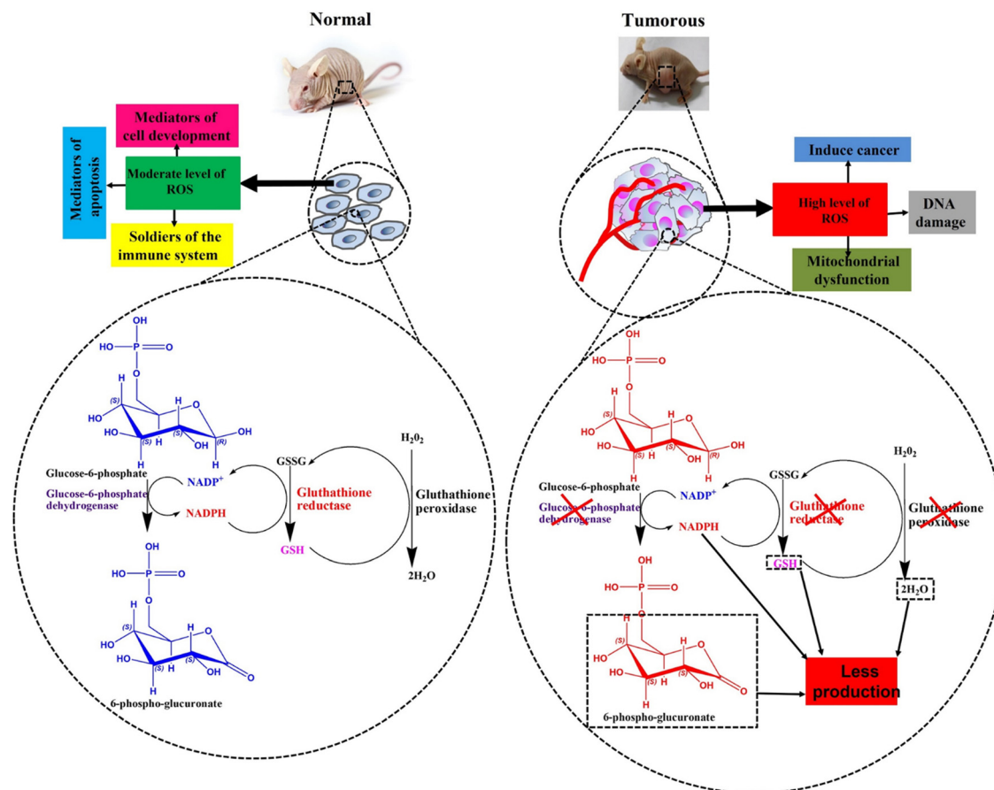
Fig. 13 Diagrammatic view of glucose-6-phosphate dehydrogenase reaction and the levels of glutathione (GSH), nicotinamide adenine dinucleotide phosphate (NADPH), and hydrogen peroxide (H 2 O 2 ) in normal and tumorous cells.
