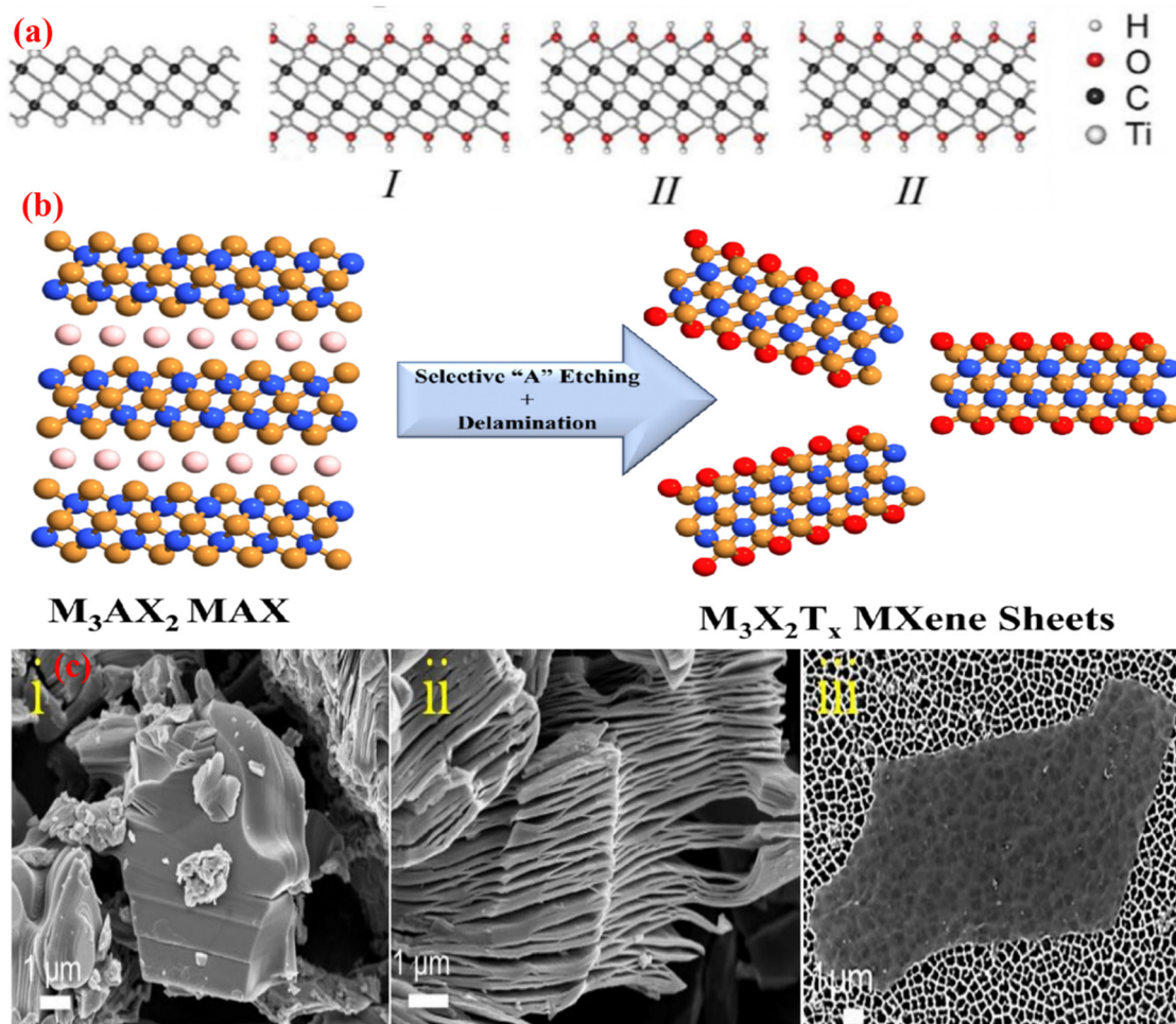
Fig. 4 (a) Configuration of the OH groups: (i) \text{Ti}_3\text{C}_2(\text{OH})_2 , (ii) \text{Ti}_2\text{C}(\text{OH})_2 , (iii) \text{Ti}_3\text{C}_2(\text{OH})_2 . Adopted with permission from ref. 73. Copyright 2012, Computational and Theoretical Chemistry, Elsevier. (b) Schematic illustration of the MXene synthesis process from the MAX phase. 74 (c) SEM images of the (i) MAX phase, (ii) Multilayer MXene, and (iii) MXene assembled flakes in a colloidal solution. Adopted with permission from ref. 62. Copyright 2017, American Chemical Society.
