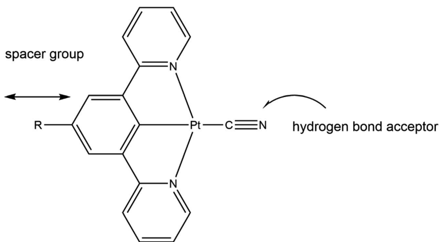
Fig. 2 The role of the substituent R and the cyanide ligand in the [\text{Pt}(\text{N}^-\text{C}(\text{R})\text{N})(\text{CN})] pincer complexes.
