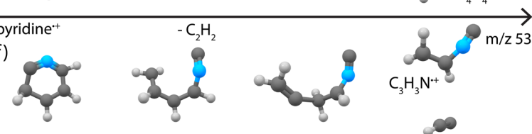
Fig. 7 Exemplary pathways for loss of (a) C 2 H 4 , (b) H 2 CN, (c) H and (d) HNC loss from alpha distonic pyridine ++ and (e) HCN and (f) C 2 H 2 loss from canonical pyridine ++ as observed in the MD/DFTB simulations at 6.74 eV internal energy of the respective cation using Set1 parameters. The arrows indicate time.
