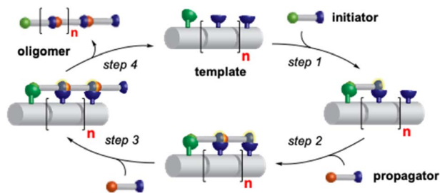
Fig. 2 Concept of catalytic length-controlled oligomerization with a linear synthetic template.
