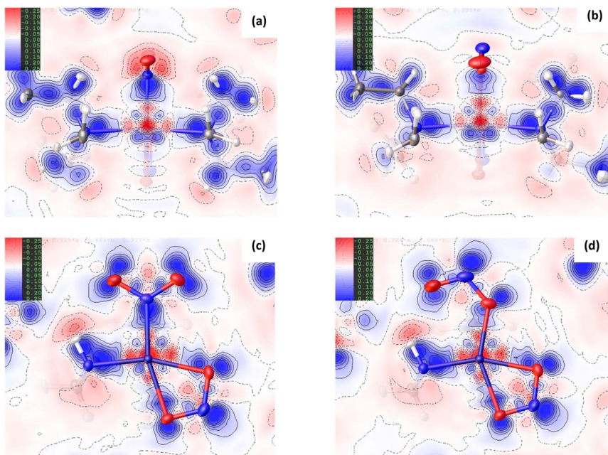
Fig. 4 2D deformation density maps for the ground state (GS) and excited state (ES) structures of complex 2 , showing the residual electron density between the non-spherical atom refinement (HAR) and a standard spherical atom model (IAM) from NoSpherA2. Blue = positive deformation density (e.g. in bonds or lone pairs), red = negative deformation density. (a) GS map in the Ni(1), N(1), N(3), N(5) plane, (b) ES map in the Ni(1), O(1A), N(3), N(5) plane, (c) GS map in the Ni(1), N(1), O(1), O(2) plane (plane of the nitro ligand), (d) ES map in the Ni(1), N(1A), O(1A), O(2A) plane (plane of the nitrito ligand).
