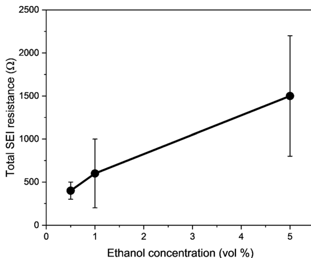
Fig. 3 A plot to show the variation in total solid electrolyte interphase (SEI) resistance (charge transfer resistance ( R_{CT} ) + SEI resistance ( R_{SEI} )) with ethanol concentration. Resistance values were obtained using potentiostatic electrochemical impedance spectroscopy (PEIS). Spectra were taken at open circuit potential after a nitrogen reduction experiment, which is at lithium plating potentials, at an amplitude of 10 mV between 200 kHz and 200 mHz. The total resistance is the sum of the resistance of the two observed semi-circles representing charge transfer resistance and SEI resistance. In general, increasing ethanol content leads to a higher total resistance ( n = 3 ).
