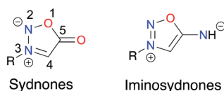
Fig. 1 General structure of sydnone and iminosydnone.
