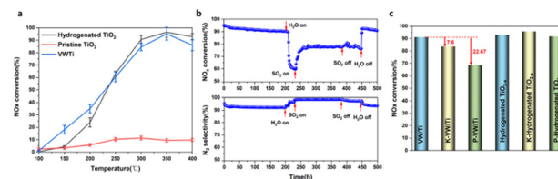
Fig. 1 \text{NH}_3 -SCR denitrification activity of the catalyst. (a) The denitrification performances of pristine \text{TiO}_2 , \text{H-TiO}_{2-x} and VW/Ti catalysts. (b) Data from 500 h durability trials with the \text{H-TiO}_{2-x} catalyst at 350 °C. (c) Tolerance of \text{K}_2\text{O} and \text{P}_2\text{O}_5 of the \text{H-TiO}_{2-x} catalyst and of commercial VW/Ti catalysts at 350 °C.
