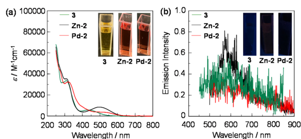
Fig. 3 (a) Photoabsorption ( 10^{-4} – 10^{-5} \text{ M} ) and (b) emission spectra ( 1.0 \times 10^{-4} \text{ M} , \lambda_{\text{ex}} = 430 \text{ nm} for 3 and 490 \text{ nm} for Zn-2 and Pd-2 ) of 3 , Zn-2 and Pd-2 in dichloromethane.
