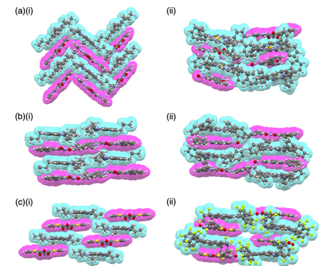
Fig. 43 Single-crystal X-ray structures of diarylnitrophenoxides: (a) (i) {}^3\text{TATA}^+ \cdot 34\text{a}^- and (ii) 22\text{a}^+ \cdot 34\text{a}^- , (b) (i) {}^3\text{TATA}^+ \cdot 34\text{b}^- and (ii) 22\text{a}^+ \cdot 34\text{b}^- and (c) (i) {}^3\text{TATA}^+ \cdot 35\text{a}^- and (ii) 22\text{d}^+ \cdot 35\text{a}^- (redrawn from cif files: 2061520, 2061524, 2061521, 2061525, 2253152 and 2253153).
