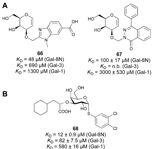
Fig. 13 Gal-8N inhibitors and their binding affinities for Gal-8N, Gal-3 and Gal-1, highlighting the selectivity for Gal-8N. (A) \beta -Galactals, (B) 3-lactoyl- \alpha - \text{D} -thiogalactopyranoside. n.b. = no binding.
