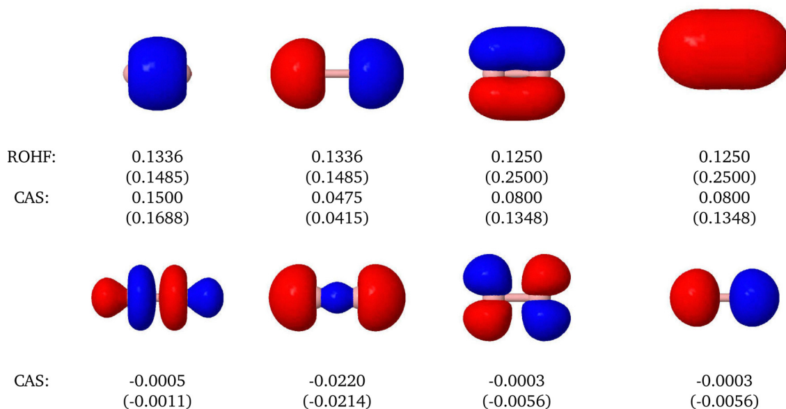
Fig. 13 |\psi| = 0.05 a.u. isosurfaces for the non-core NAOs in the B2 and C2 molecules. The numbers below correspond to their respective occupations n_i^{ab} at the ROHF and CAS levels, with a 6-311G(d,p)++ basis set. C 2 data in parenthesis. Reproduced from ref. 256. Copyright 2015 John Wiley and Sons, Inc.
