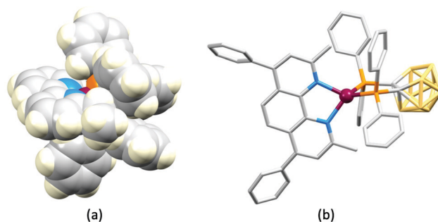
Fig. 20 (a) Structure of the cation in [Cu(BIPHEP)(6-Etbpv)]PF 6 in space-filling representation (CSD refcode WOXHEZ). (b) Structure of [Cu(dppnc)(2,9-Me 2 -4,7-Ph 2 -phen)] (CSD refcode MUJXOG) with H atoms omitted.
