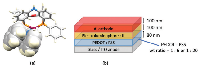
Fig. 19 (a) Structure of the cation in [Cu(HN-xantphos)(6-Mebpy)][PF 6 ] with the Ph...bpy \pi -stacking interaction shown in space-filling representation (CSD refcode TUHXC). (b) Architecture of the LECs containing [Cu(BnN-xantphos)(6,6'-Me 2 bpy)][PF 6 ]; IL = [EMIM][PF 6 ], and Cu-iTMC; IL molar ratio = 4 : 1; two compositions of the hole-injection layer were used; LECs were driven using a pulsed current.
