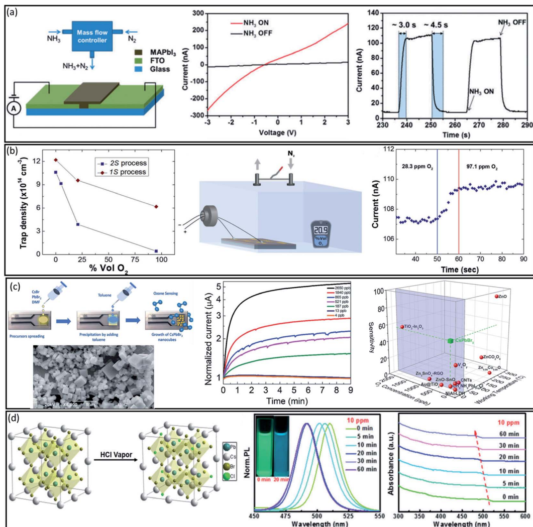
Fig. 8 (a) Schematic illustration of the resistance measurement set-up for \text{NH}_3 gas sensing of an \text{MAPbI}_3 film, the I - V curves and enlarged view of I - V curves during \text{NH}_3 ON and OFF at room temperature. Reproduced with permission from ref. 126, Copyright 2015 the Royal Society of Chemistry. (b) The number of charge traps for 1S and 2S perovskite films at different oxygen concentrations, the schematic of the experimental setup for \text{O}_2 sensing characterization and the real-time current change corresponding to a 70 ppm \text{O}_2 variation in the sample atmosphere. Reproduced with permission from Ref.127, Copyright 2014 John Wiley and Sons. (c) Schematic illustration of ozone sensor fabrication and the SEM image of \text{CsPbBr}_3 nanocubes, the electrical response of the \text{CsPbBr}_3 sensor upon applying various ozone concentrations and ozone sensitivity of a \text{CsPbBr}_3 sensor compared to other types of sensors. Reproduced with permission from ref. 129, Copyright 2019 the Royal Society of Chemistry. (d) Schematic of the anion-exchange reaction between gaseous \text{HCl} and \text{CsPbBr}_3 perovskite, the PL spectra of exposed \text{CsPbBr}_3 nanocrystals to \text{HCl} for different times (insets show the photograph of the visual changed colour of sample exposed to 10 ppm \text{HCl} for 20 minutes) and the UV-vis absorption spectra of \text{CsPbBr}_3 nanocrystals exposed to 10 ppm \text{HCl} for different times. Reproduced with permission from ref. 130, Copyright 2017 the Royal Society of Chemistry.
