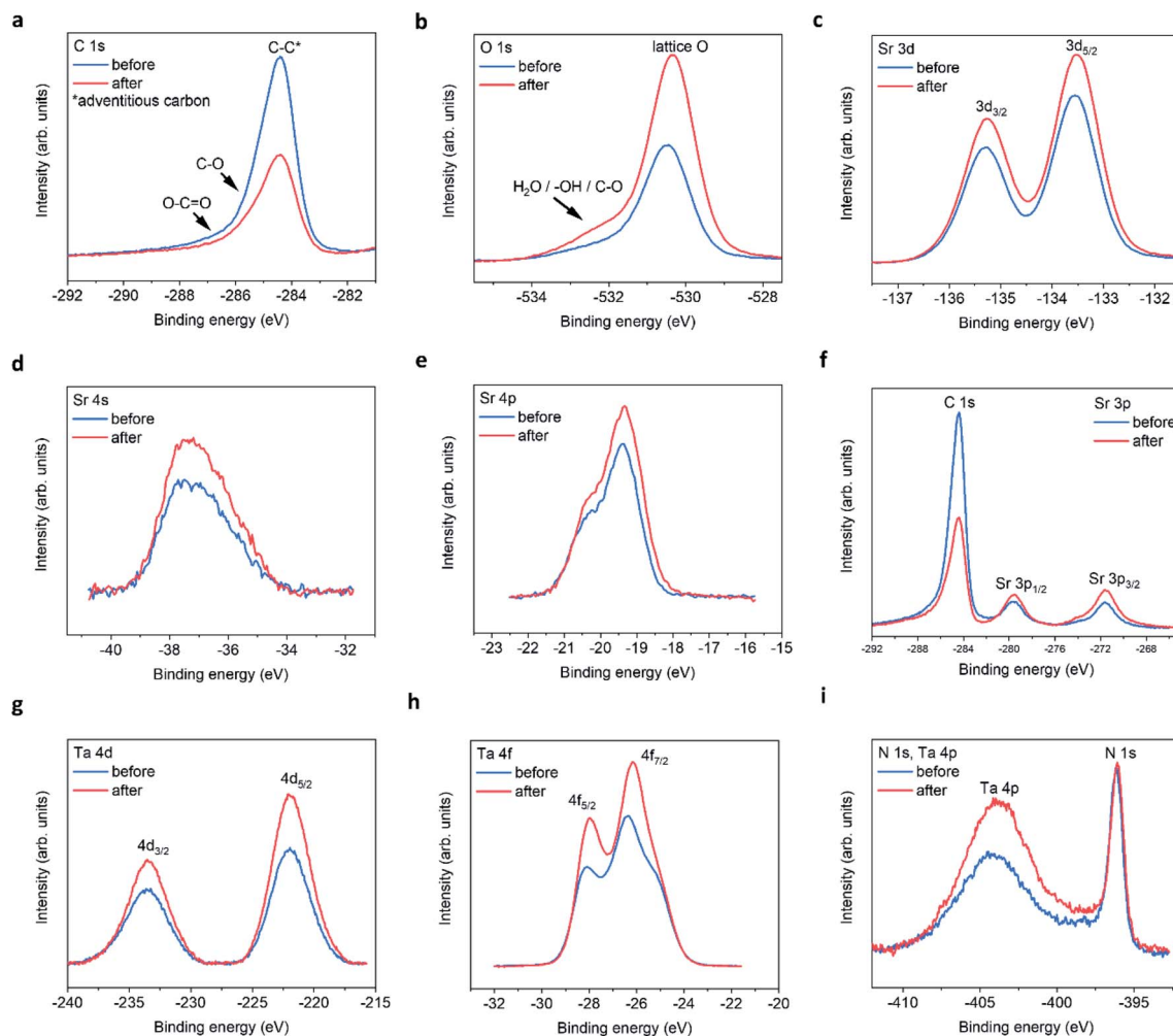
Fig. 3 STON thin film XPS spectra before and after PEC. (a) C 1s, (b) O 1s, (c) Sr 3d, (d) Sr 4s, (e) Sr 4p, (f) Sr 3p, (g) Ta 4d, (h) Ta 4f, (i) N 1s and Ta 4p edges.
