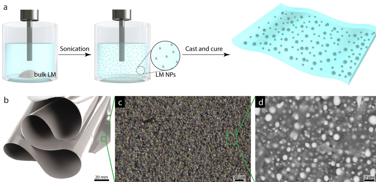
Fig. 1 Liquid metal soft composites. (a) Schematics showing the fabrication of LM nanodroplets using probe sonication. (b) Photograph showing the soft, flexible nature of the LM composites. (c) Optical micrograph and (d) SEM image of a composite showing LM microstructure.
