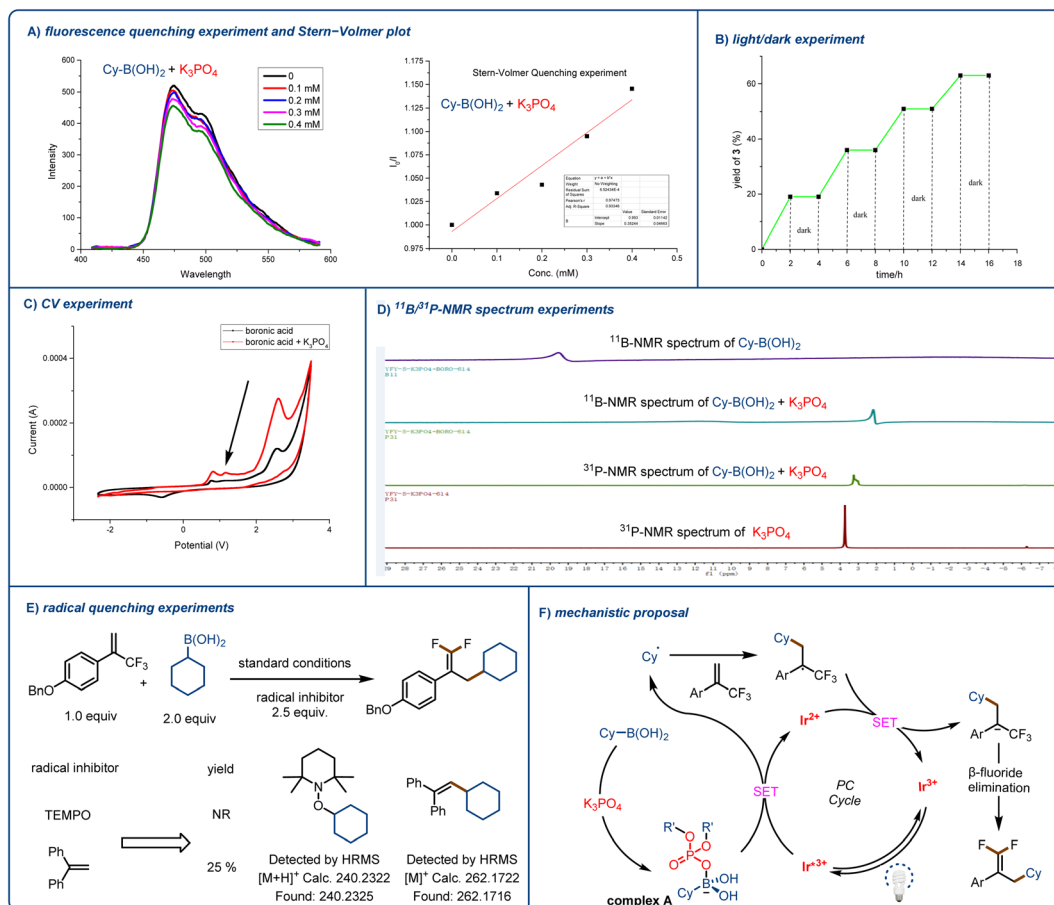
Fig. 2 Mechanistic experiments. (A) Fluorescence quenching experiment and Stern–Volmer plot confirming that the excited state of the photocatalyst was quenched by the cyclohexylboronic acid– \text{K}_3\text{PO}_4 complex. (B) Light/dark experiment. (C) Cyclic voltammograms showing lowering of the cyclohexylboronic acid oxidation potential by \text{K}_3\text{PO}_4 . (D) ^{11}\text{B} NMR and ^{31}\text{P} NMR spectra in \text{D}_2\text{O} (0.5 mL). (E) Radical quenching experiments. (F) Proposed mechanism, \text{R}' = \text{cyclohexylboronic acid} .
