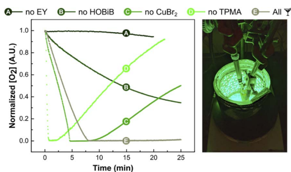
Fig. 5 Oxygen concentration measurements. Reactions conditions: [HOBiB]/[EYH 2 ]/[CuBr 2 ]/[TPMA] = 1/0.01/0.2/0.6, [HOBiB] = 1.5 mM, in PBS with DMSO (10% v/v), irradiated for 30 min under green LEDs (520 nm, 9.0 mW cm -2 ) in an open vial with stirring at 500 rpm.
