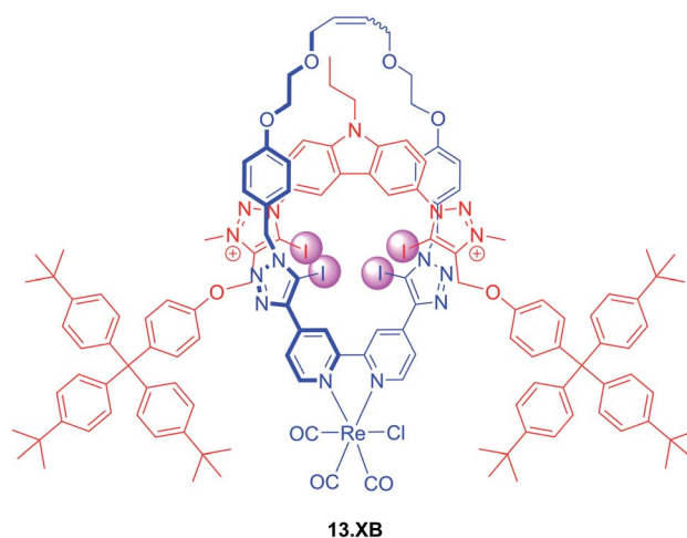
Fig. 16 All XB Re(i)(CO) 3 Cl-containing [2]rotaxane 13.XB for selective fluorescent halide sensing in ACN/ \text{H}_2\text{O} mixtures.
