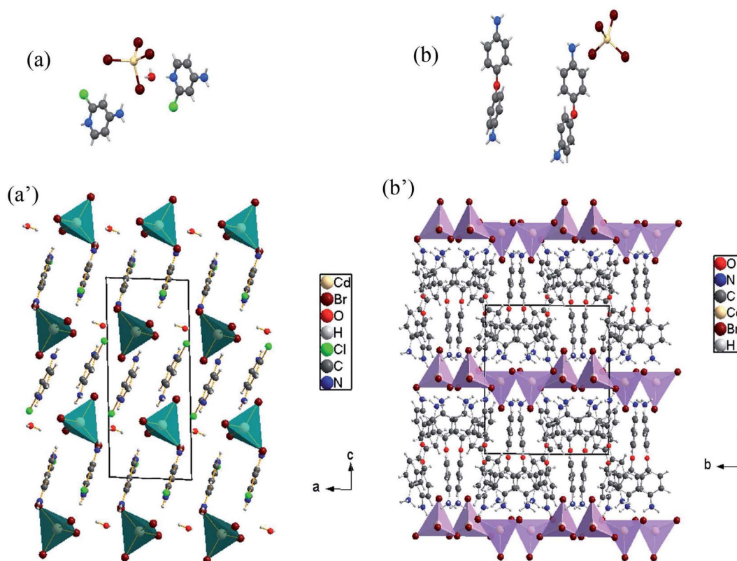
Fig. 1 Asymmetric units and structure projection of \text{CdACP} ((a) and (a')) and \text{CdODA} ((b) and (b')).
