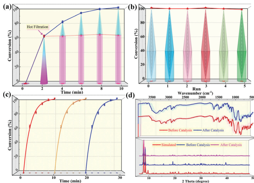
Fig. 5 (a) Hot filtration experiment using 1 for the catalytic oxidation of MPS. (b) Cycling experiments involving the oxidation of MPS using spent 1 . (c) Continuous cycling experiments involving the oxidation of MPS using 1 . (d) The FTIR spectra and PXRD patterns of fresh and spent catalyst 1 .
