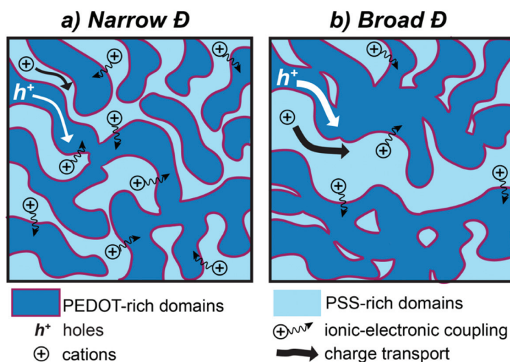
Fig. 8 Schematic of the proposed interpretation for the difference in OECT performance of PEDOT:PSS based on PSS size distribution ( \mathcal{D} ). (a) PEDOT:PSS with narrow PSS \mathcal{D} . (b) PEDOT:PSS with broad PSS \mathcal{D} . The broad dispersity of PSS leads to larger domain sizes making it easier for holes (white arrow) to transport through the PEDOT-rich domains and cations (black arrow) to transport through the PSS-rich domains. Ionic-electronic coupling (wavy arrows) is lower at broad \mathcal{D} due to a reduction in the interfacial area (in red) between PEDOT- and PSS-rich domains.
