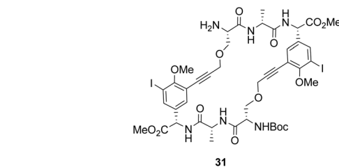
Fig. 12 By-product cyclic dimer 31.
