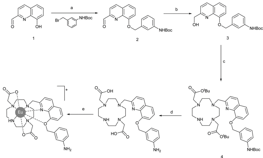
Scheme 2 Synthesis of EumNH2. Conditions: (a) K_2CO_3 , DMF, rt, 2 h, 88%; (b) NaBH_4 , MeOH, 0 °C to rt, 55%; (c) i) MsCl , Et_3N , DCM, 0 °C to rt, (ii) DO2A tert -butyl ester, K_2CO_3 , MeCN, 60 °C, 18hr, 71% over two steps; (d) 3 : 1 DCM/TFA, 18 h, quant; (e) EuCl_3 \cdot 6H_2O , water, 60 °C, pH \geq 7.2, prep HPLC, 9%.
