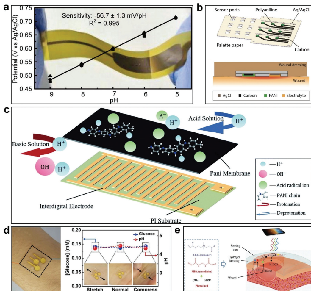
Fig. 2 Some pH sensors. (a) A WO 3 -based flexible pH sensor without softness or stretchability. 68 This figure has been reproduced from ref. 68 with permission from the American Chemical Society; copyright: 2014. (b) A low-cost pH sensor array for wound monitoring. 69 This figure has been reproduced from ref. 69 with permission from Elsevier B.V.; copyright: 2016. (c) A flexible pH sensor based on conductive polyaniline membrane. 71 The sensor is hard and non-stretchable, limiting its long-term wearability. This figure has been reproduced from ref. 71 with permission from the Royal Society of Chemistry; copyright: 2020. (d) A stretchable and soft electrochemical sweat sensor attached to skin for glucose and pH detection. 72 The sensor has good adhesion to the skin and can be directly attached to the skin. In addition, the sensor is able to stretch and compress with the skin due to its softness and stretchability. This figure has been reproduced from ref. 72 with permission from the American Chemical Society; copyright: 2018. (e) A multifunctional pro-healing amphoteric ionic hydrogel for the simultaneous monitoring of pH and glucose for diabetic wound therapy. 76 The ionic hydrogel can conformally attach to the skin due to its good adhesion properties and low elastic modulus. This figure has been reproduced from ref. 76 with permission from WILEY-VCH Verlag GmbH & Co. KGaA; copyright: 2019.
